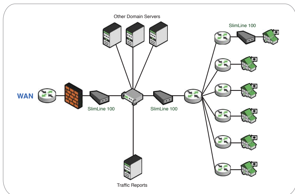
Figure 1: Gilmer County School System Network
